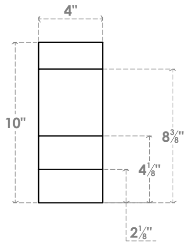
FRONT PROFILE
